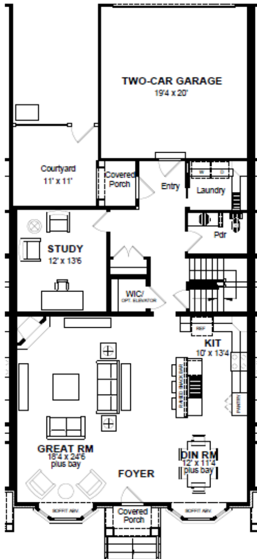
BROWNSTONE CENTER UNIT B 1340 SF FIRST FLOOR W - 31' D - 70'
