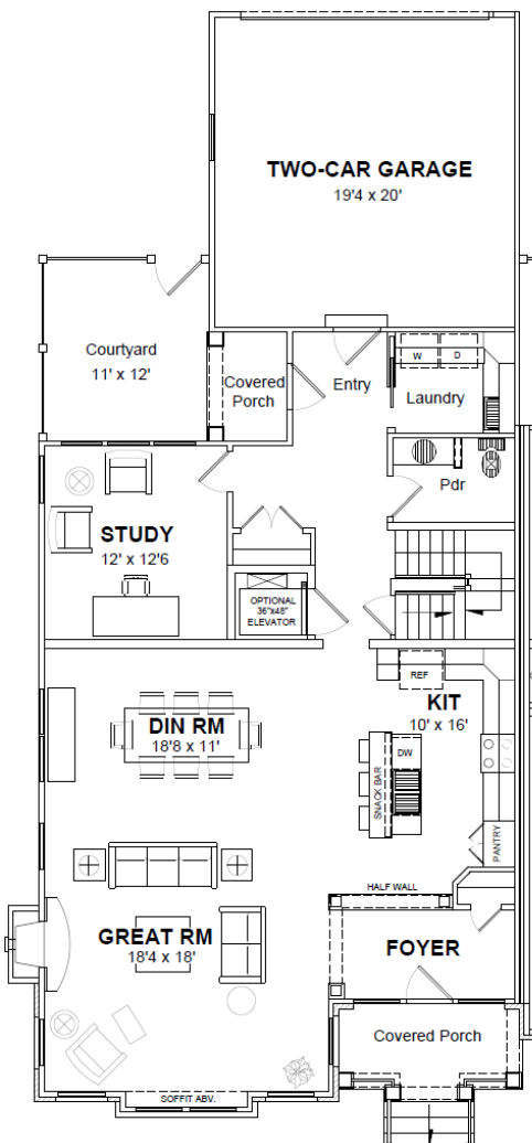
BROWNSTONE END UNIT A 1359 SF FIRST FLOOR
