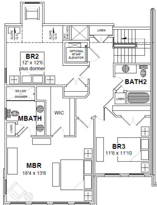
BROWNSTONE END UNIT A 1123 SF SECOND FLOOR
