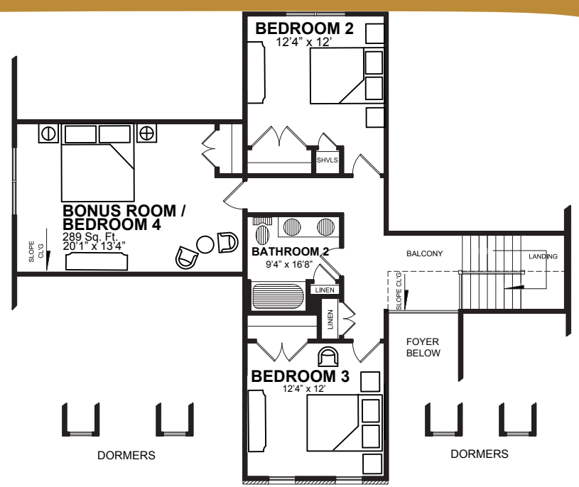
SECOND FLOOR 955 Square Feet BONUS ROOM / BEDROOM 4
