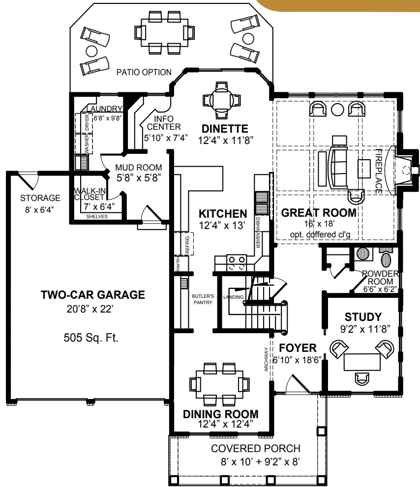
FIRST FLOOR 1,388 Square Feet
