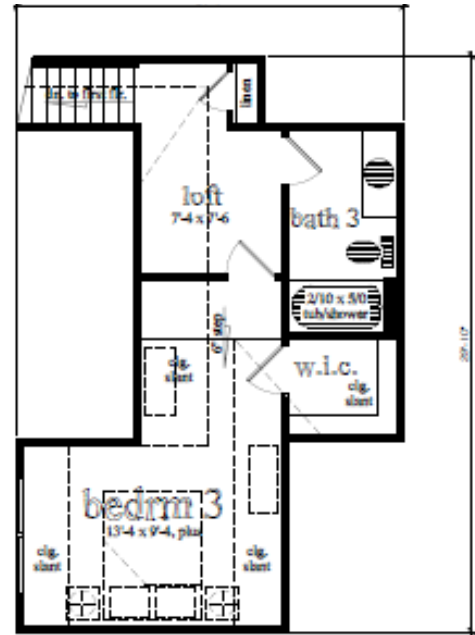
second floor plan 428 s.f.
