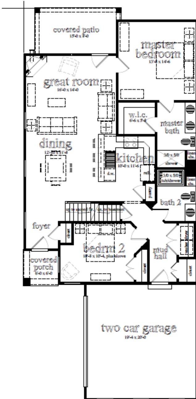
first floor plan 1298 s.f.
